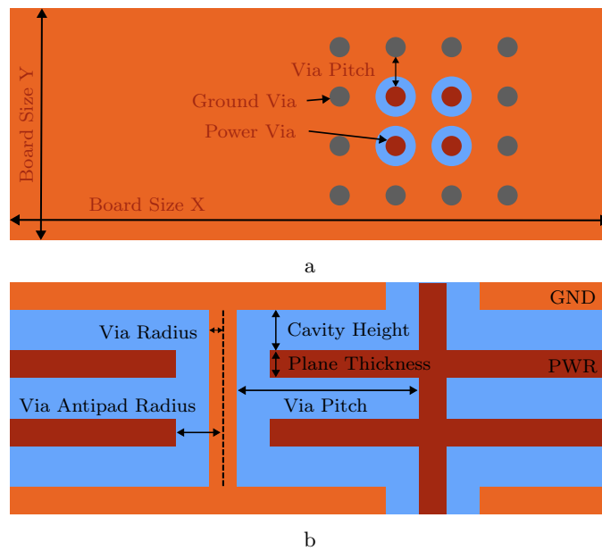
Figure 1: a) Top view of the printed circuit board (PCB), b) side view of the printed circuit board (PCB). The parameters are named as found in the data files. The via array consists of 4 power vias surrounded by ground vias. The vias have the same properties as specified in the parameter.csv file, e.g. via radius.
